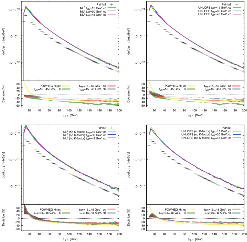
Figure III.6: Transverse momentum of the hardest jet, for H-boson production in pp collisions at E_{CM} = 7000 GeV, when merging up to two additional partons at LO, and zero and one additional parton at NLO. Jets were defined with the k_{\perp} -algorithm, with k_{\perp,min} = 10 GeV. Multi-parton interactions and hadronisation were excluded. The lower inset shows the deviation from PYTHIA8. The band labelled “POWHEG W+jet” is given by the envelope of varying the renormalisation scale in the POWHEG-BOX program between \frac{1}{2}M_Z, \dots, 2M_Z , and the factorisation scale between \frac{1}{2}M_H, \dots, 2M_H . The upper panels show the results for using the zero-jet K -factor (i.e. K = \frac{\sigma_{B_0}}{\sigma_{B_0}} ) throughout the NLO merging procedures. The lower panel show the result when not using any K -factor (i.e. K = 1 ). Left columns: Results of NL 3 . Right columns: Results of UNLOPS.
