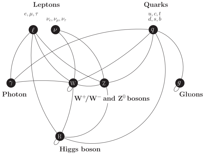
Figure i.1 : The Standard Model of particle physics, with lines indicating interactions. Electrically charged particles exchange photons. Leptons further interact through W- and Z-boson exchange, as do the quarks, which also communicate through gluon exchange. Every massive particle interacts with the Higgs field. Gluons interact among themselves, as do W- and Z-bosons, and the Higgs boson.
