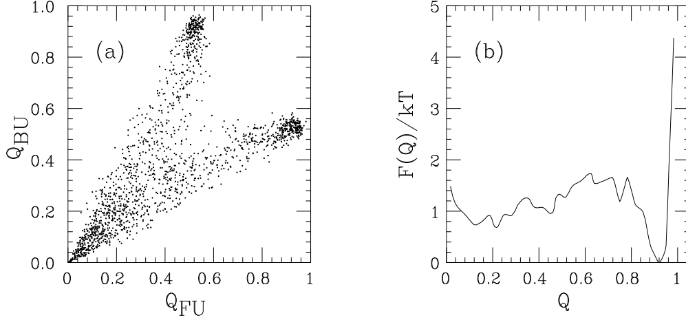
Figure 6: (a) Q_{FU}, Q_{BU} (see Eq. 8) scatter plot at the specific heat maximum ( kT = 0.658 ). (b) Free energy F(Q) as a function of Q = \max(Q_{FU}, Q_{BU}) at the same temperature.
