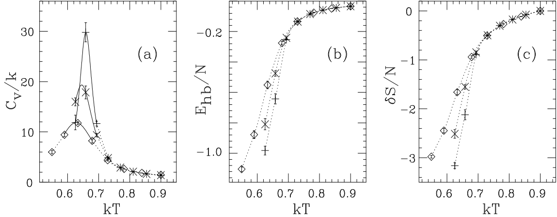
Figure 4: Thermodynamic functions against temperature for the sequences 1H ( \diamond ), 2H ( \times ) and 3H ( + ) in Table 3. (a) Specific heat C_v = (\langle E^2 \rangle - \langle E \rangle^2) / NkT^2 , N being the number of amino acids. (b) Hydrogen-bond energy per amino acid, E_{\text{hb}}/N . (c) Chain entropy per amino acid, \delta S/N = [S - S(kT = 0.9)]/N . The full lines in (a) represent single-histogram extrapolations [35]. Dotted lines are drawn to guide the eye.
