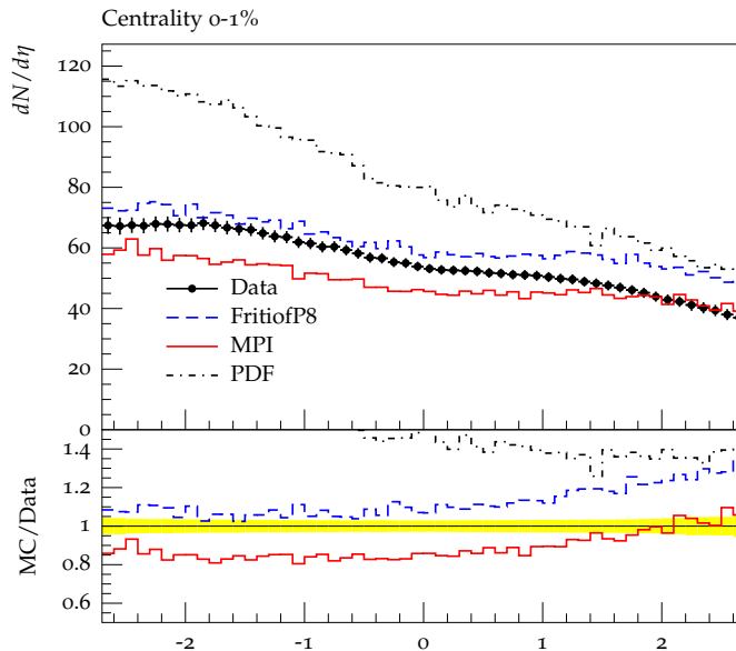
Figure 12: Pseudo-rapidity distribution of charged particle multiplicity for centrality 0 – 1% compared to three different ways of estimating the number of MPIs, giving an estimate of the method uncertainty.
