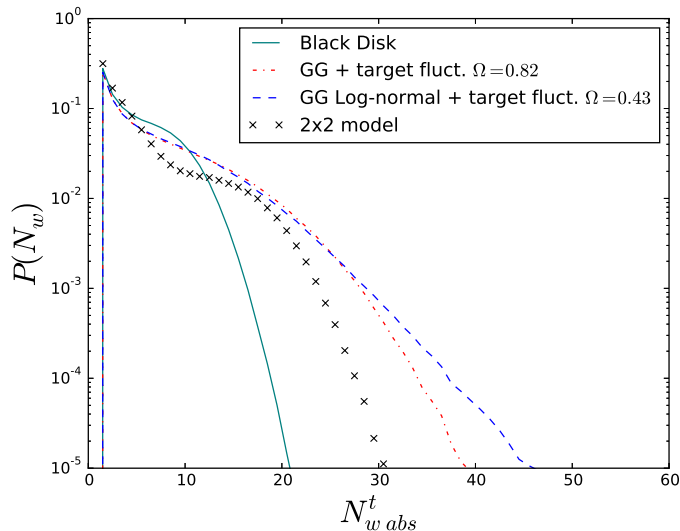
Figure 6: Distribution in the number of absorptively wounded nucleons, N_{w\text{abs}}^t , in pPb events at \sqrt{s_{NN}} = 5 TeV, for a Glauber black disk, the GG model with two parametrisation of P(\sigma) , corrected using the 2 \times 2-disk model, along with the 2 \times 2-disk model itself. All models have been fitted to reproduce relevant measured (semi-) inclusive cross sections.
