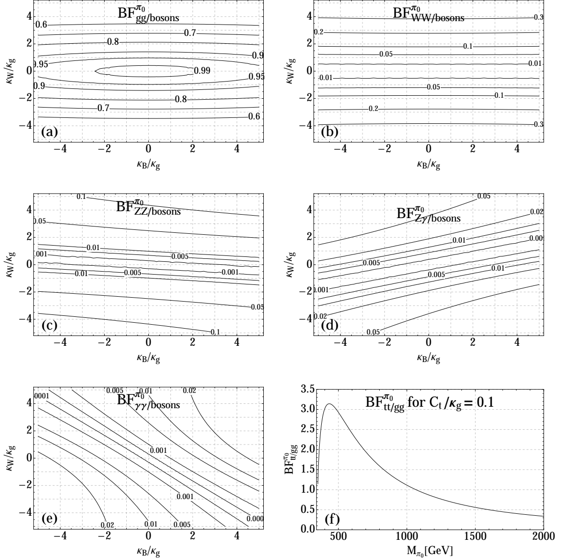
FIG. 2: Ratios of the \pi_0 decay channels. In (a) - (e) we show BF_{XY/bosons} in the \kappa_W/\kappa_g vs. \kappa_B/\kappa_g plane, evaluated at M_{\pi_0} = 1 TeV (the mass-dependence mainly enters through the running of \alpha_s ). In (f), BF_{tt/gg} is plotted as a function of M_{\pi_0} for C_t/\kappa_g = 0.1 ( BF_{tt/gg} scales like (C_t/\kappa_g)^2 ).
