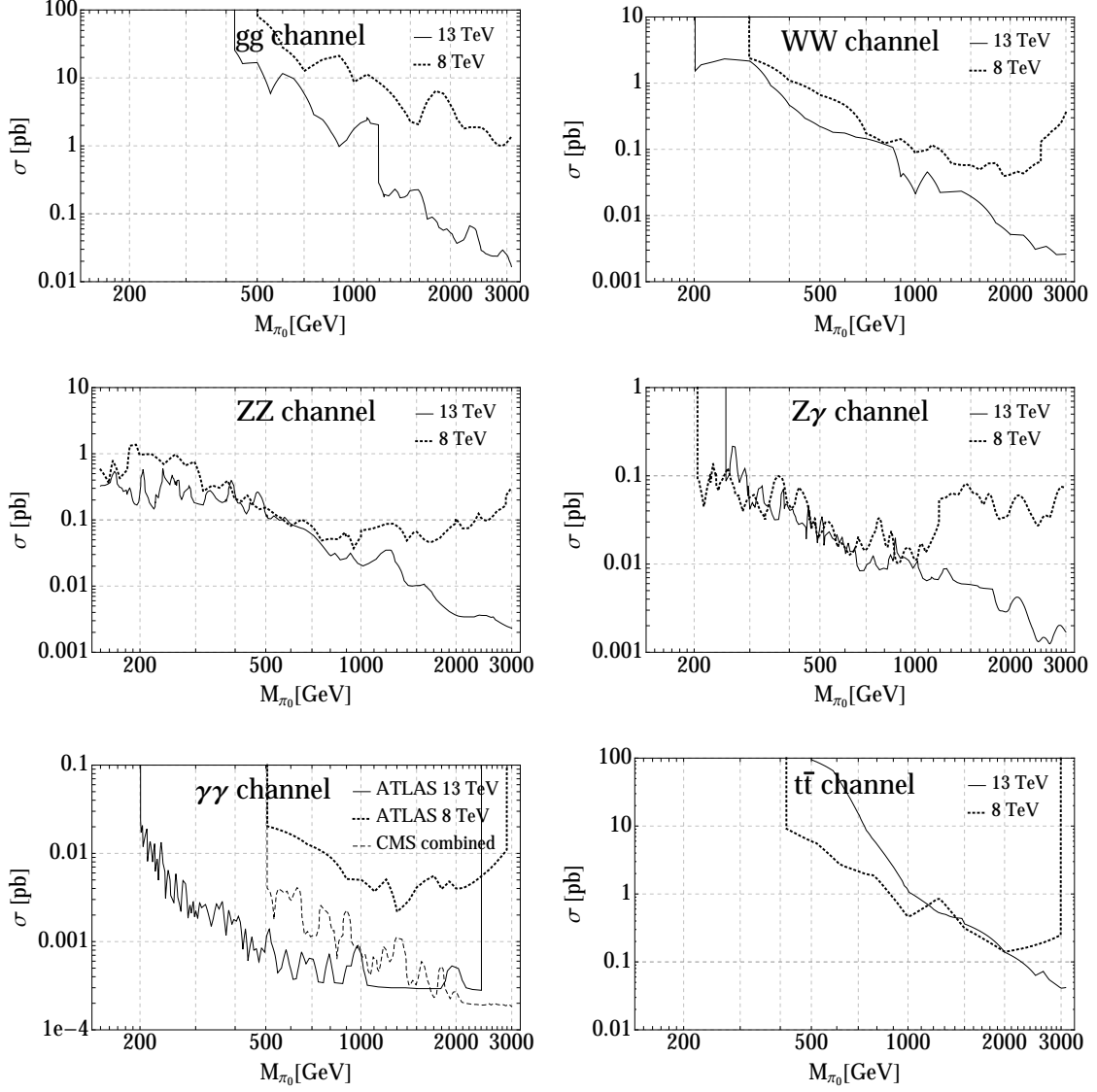
FIG. 3: Bounds on the di-boson and t\bar{t} channels from 13 TeV searches and 8 TeV searches on the 13 TeV production cross section times branching ratio. 8 TeV bounds have been rescaled by the ratio of 13 TeV / 8 TeV production cross section for gluon fusion in order to allow direct comparison. For the di-photon channel, we show the combined results from 13 and 8 TeV determined by CMS as well as the (still separate) 8 and 13 TeV search results by ATLAS.
