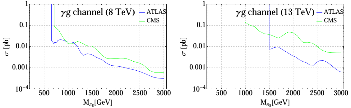
FIG. 16: Bounds on g\gamma channel from 8 and 13 TeV searches.
