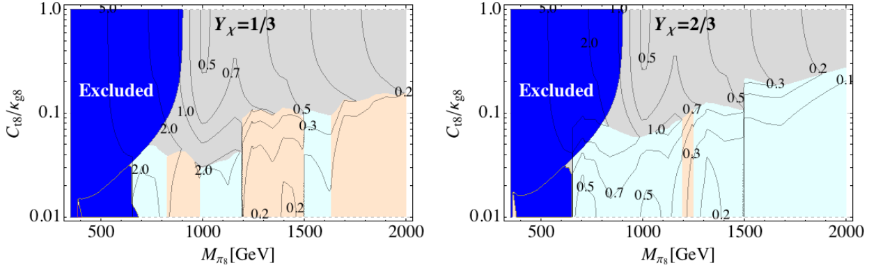
FIG. 11: Bounds on the production cross section (in pb) in the C_{t8}/\kappa_{g8} vs. M_{\pi_8} plane for Y_\chi = 1/3 (left) and Y_\chi = 2/3 (right). The blue region is excluded by octet pair production searches. The currently strongest bounds arise from the t\bar{t} channel (gray regions), gg channel (orange regions) and the g\gamma channel (light-cyan regions).
