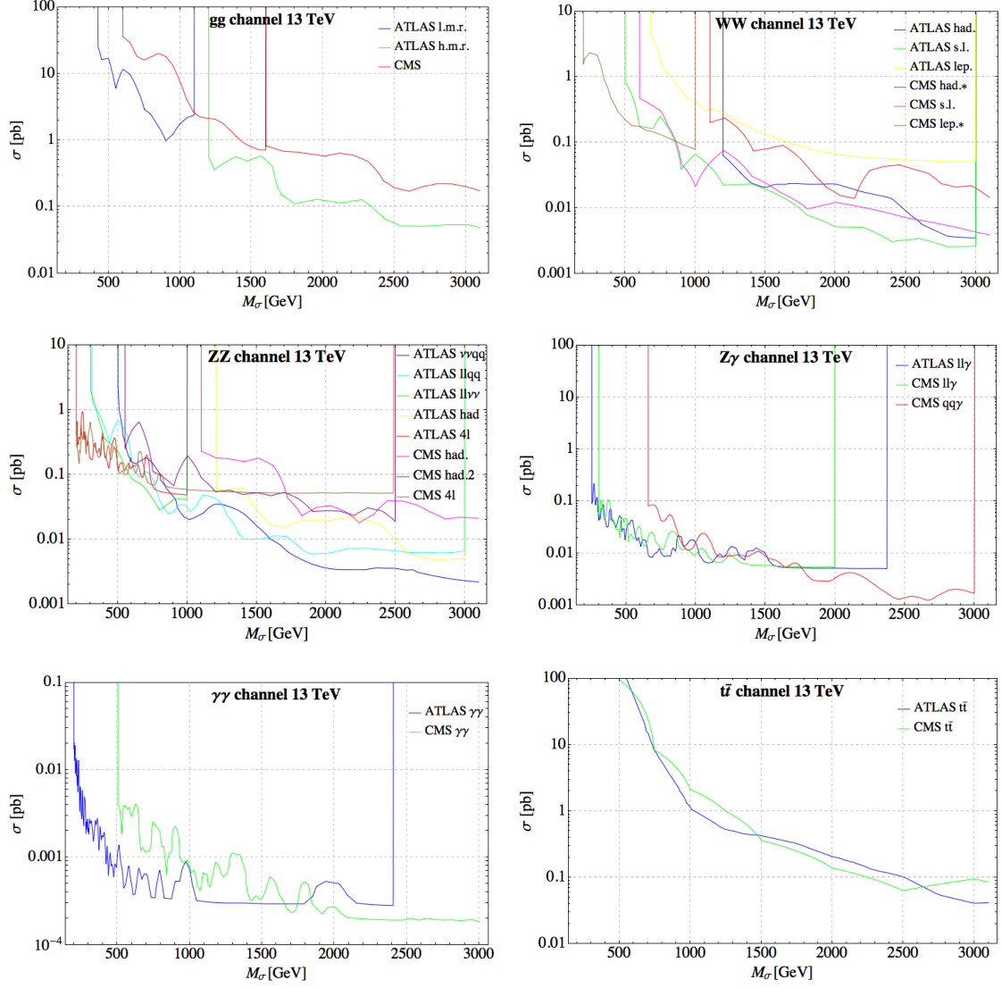
FIG. 15: Bounds on the di-boson and t\bar{t} channels from 13 TeV searches.
