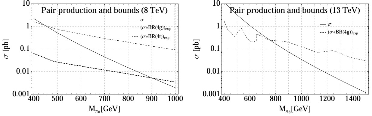
FIG. 8: Color octet pair production cross section (from Ref. [57]) and the current bounds on \sigma \times BR(pp \rightarrow \bar{t}t\bar{t}t) [107, 108] and \sigma \times BR(pp \rightarrow 4j) [105] for \sqrt{s} = 8 TeV (left) and \sigma \times BR(pp \rightarrow 4j) [106] for \sqrt{s} = 13 TeV (right).
