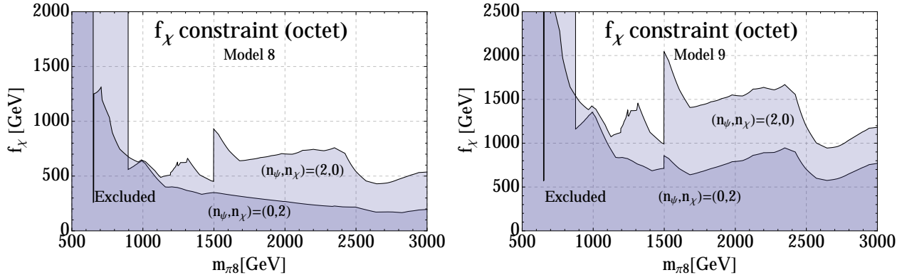
FIG. 12: Lower bounds on f_\chi from LHC searches sensitive to the octet, in the case of model M8 (Left) and M9 (Right). The two lines correspond to the two choices of charges (2, 0) and (0, 2) .
