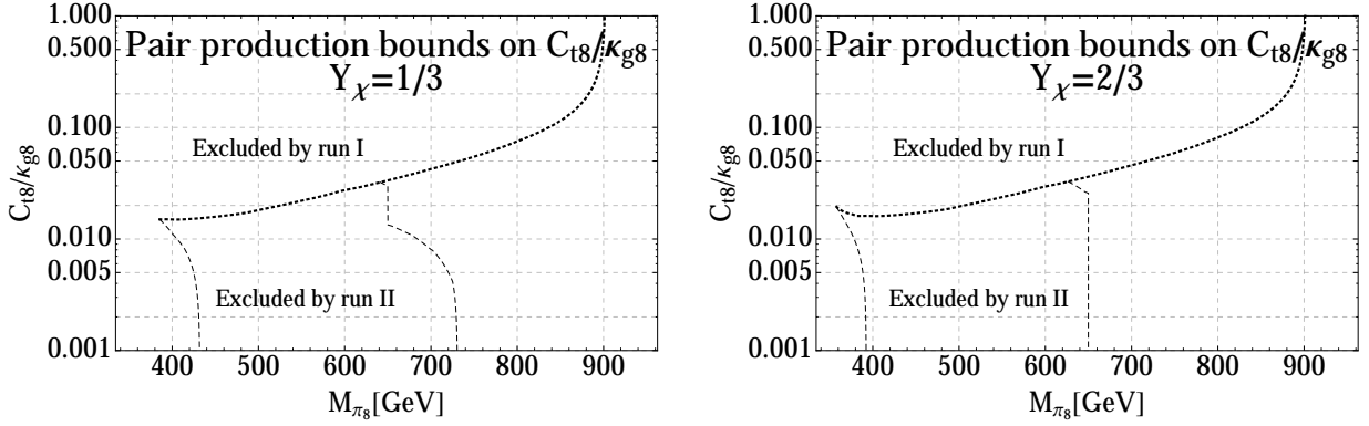
FIG. 9: Bounds on C_{t8}/\kappa_{g8} as a function of M_{\pi_8} from 4t and 4j searches. The parameter regions excluded by 8 and 13 TeV data are also shown, as they do not depend on the overall value of the couplings.
