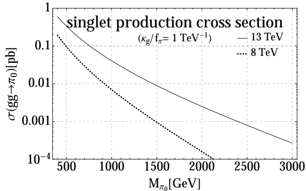
FIG. 1: Production cross section of a pseudo-scalar \pi_0 with coupling \kappa_g/f_\pi = 1 \text{ TeV}^{-1} from gluon fusion as a function of its mass M_{\pi_0} at the LHC.
