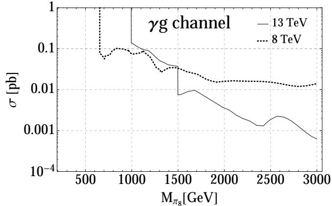
FIG. 10: Bounds from excited quark searches (final state: \gamma j ) at 13 TeV [111, 113] and 8 TeV [110, 112] which we use to constrain the \gamma g channel of color-octet decay. The 8 TeV limits are rescaled to the value of the 13 TeV cross section times branching ratio (8 TeV bounds have been appropriately rescaled by the ratio of 13 TeV / 8 TeV production cross section for gluon fusion).
