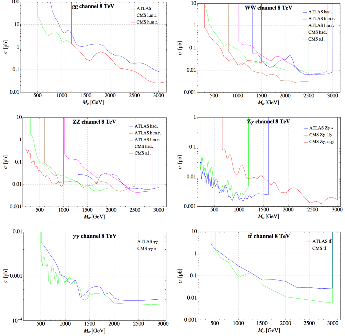
FIG. 14: Bounds on the di-boson and t\bar{t} channels from 8 TeV searches.
