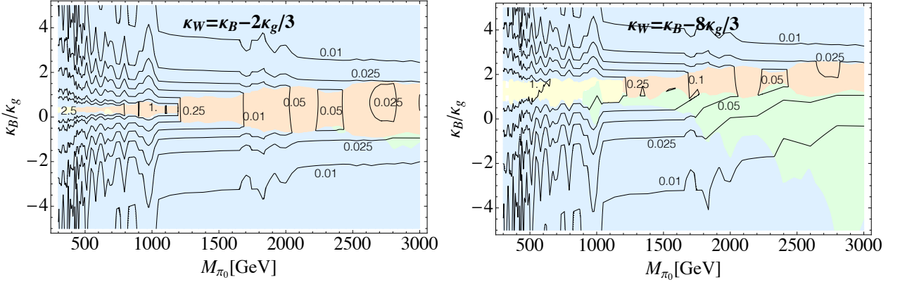
FIG. 5: Bounds on \sigma_{13} \times BR_{\text{bosons}} (in pb) in the mass vs. \kappa_B/\kappa_g plane. We present the results for two particular lines in the \kappa_B/\kappa_g vs. \kappa_B/\kappa_g parameter plane. The relation \kappa_W = \kappa_B - \frac{2}{3}\kappa_g (left plot) is realized for a and \eta' of all models with Y_\chi = 1/3 discussed in Sec. II, while the relation \kappa_W = \kappa_B - \frac{8}{3}\kappa_g (right plot) is realized for a and \eta' of all models with Y_\chi = 2/3 . The colored areas indicate the decay channel which with current data yields the strongest constraint: gg (orange), WW (green), Z\gamma (yellow), or \gamma\gamma (blue). The strongly varying bounds in the area below \sim 1 TeV are a direct consequence of the strong variation with mass of the experimental constraints (mainly the di-photon) as evident in Fig. 3.
