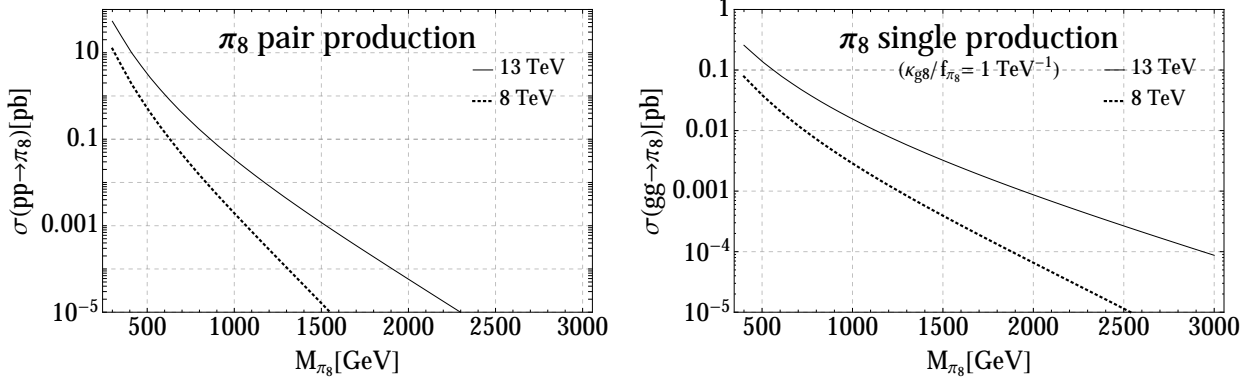
FIG. 7: Production cross sections of the color octet pNGB as a function of M_{\pi_8} at 8 and 13 TeV LHC. Left: Pair-production via QCD interactions. Right: single-production (through gluon fusion) for \kappa_{g8}/f_{\pi_8} = 1 \text{ TeV}^{-1} . Single production scales with (\kappa_{g8}/f_{\pi_8})^2 .
