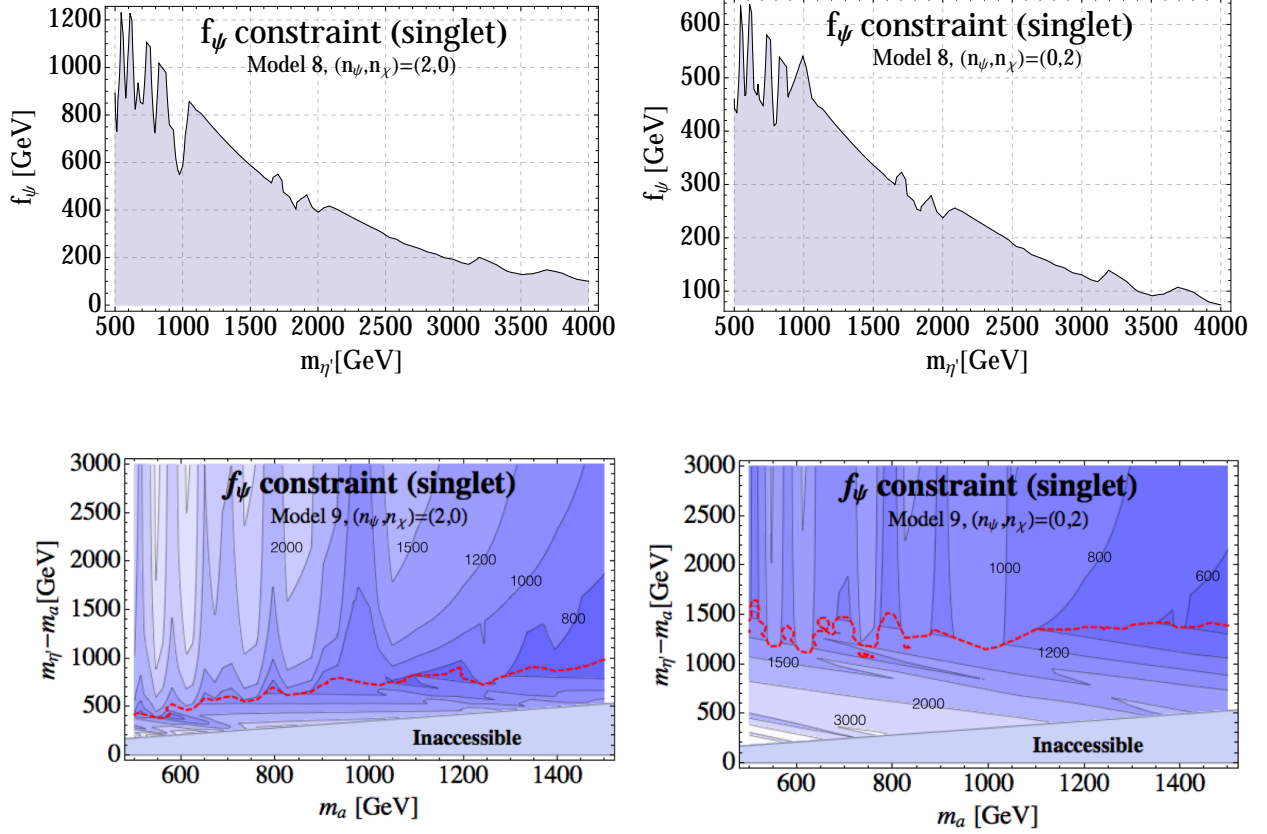
FIG. 13: Lower bound on f_\psi (in GeV) from LHC searches sensitive to singlets. Top row shows results for model M8, as a function of m_{\eta'} . Bottom row for model M9, as a function of the two masses m_a and m_{\eta'} . The Left (Right) plots corresponds to charges (\pm 2, 0) ((0, \pm 2)) . The red line in the M9 plots delimits the region where the bound is driven by the \eta' (below) from the a one (above).
