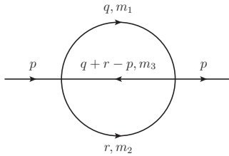
Figure 1: Sunset diagram
