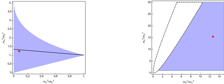
Figure 2: Region of convergence for results presented in Appendix B (blue area).
