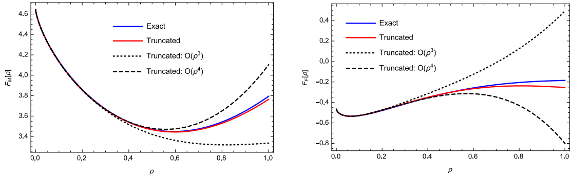
Figure 4: F_M (left) and F_F (right) plotted against \rho using exact and truncated sunset integral values, as well as expansions of the latter upto \mathcal{O}(\rho^3) and \mathcal{O}(\rho^4) .
