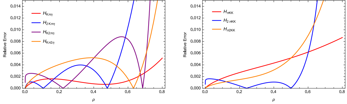
Figure 3: Relative errors of the truncated sunset kaon (left) and eta (right) integrals.
