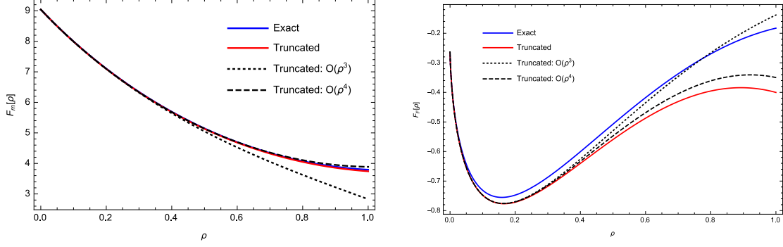
Figure 5: F_m (left) and F_f (right) plotted against \rho using exact and truncated sunset integral values, as well as expansions of the latter upto \mathcal{O}(\rho^3) and \mathcal{O}(\rho^4) .
