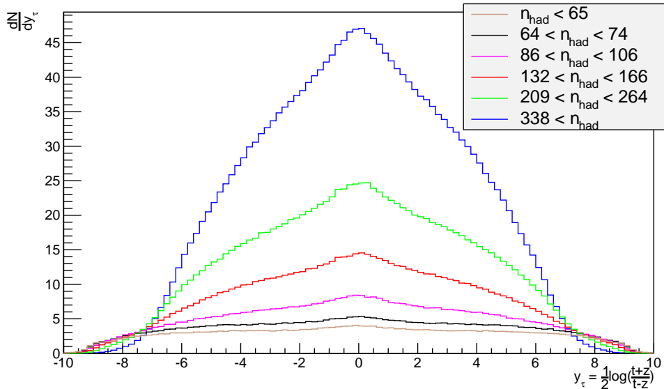
Figure 23: Longitudinal spectra for 13 TeV pp collisions and different multiplicity ranges.
