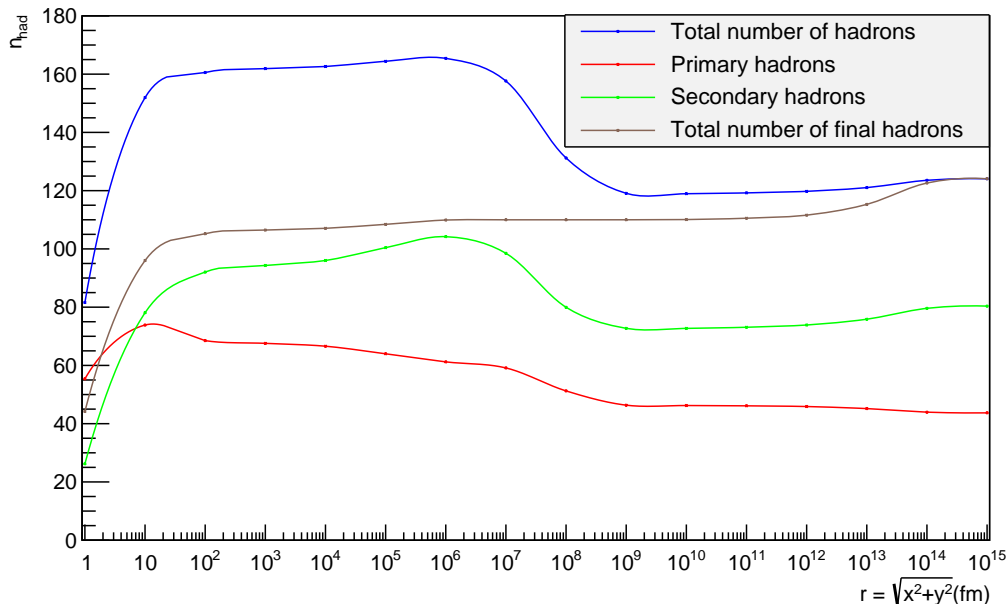
Figure 21: Hadron number per event as a function of radius for 13 TeV pp collisions
