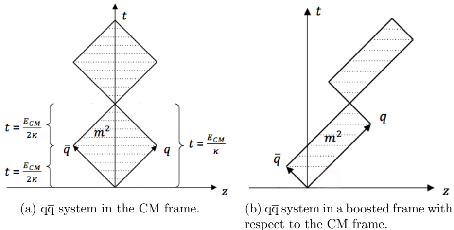
Figure 2: The motion of a q\bar{q} system, with massless q and \bar{q} .
