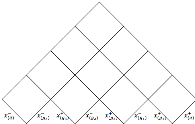
Figure 8: The parameter plane picture for a multiparton system composed by five partons.
