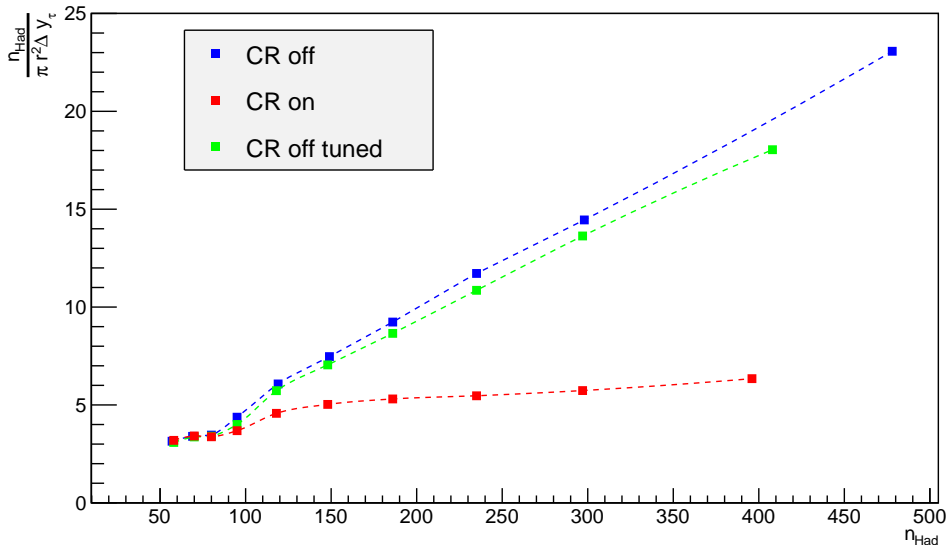
Figure 26: Hadron density as a function of multiplicity for pp collisions at 13 TeV. The red, blue and green curves represent the three different models with and without colour reconnection, also included in Fig. 25.
