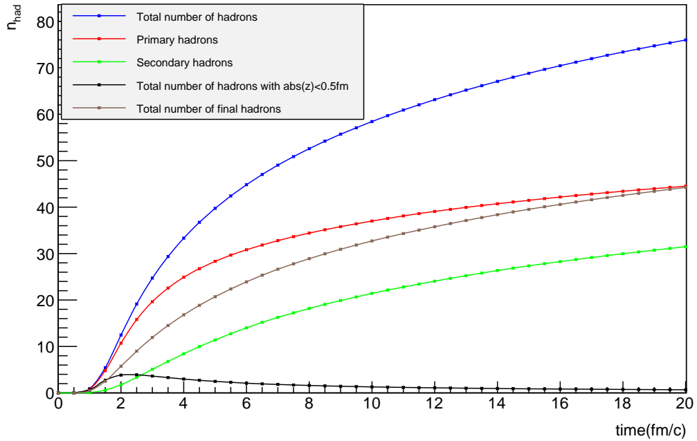
Figure 19: Hadron number per event as a function of time, up until t = 20 fm, for pp collisions at \sqrt{s} = 13 TeV.
