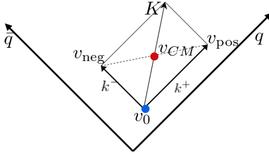
Figure 32: Final region of a q\bar{q} system. The origin of the region is represented by v_0 while v_{\text{CM}} stands for the location of the CM of the region. The four-momentum of the final region is defined as K . As in other cases, v_{\text{pos}} and v_{\text{neg}} represent the old breakups.
