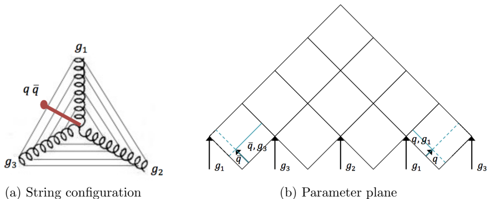
Figure 12: The string configuration and the corresponding parameter plane for a three gluon-loop topology. In the two initial endpoint regions the full lines indicate the “active area”, and the dashed ones the complementary excluded one.
