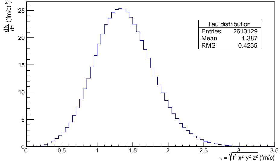
Figure 18: Invariant time \tau distribution of primary hadrons in q\bar{q} systems.
