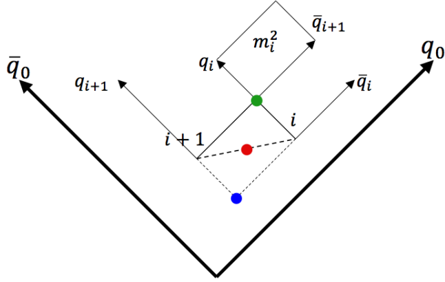
Figure 9: Hadron formation in a q\bar{q} system. The blue, red and green dots represent the “early”, “middle” and “late” definitions of hadron production points, respectively.
