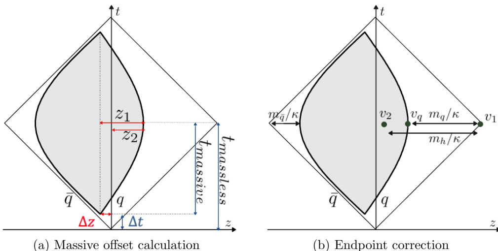
Figure 13: Massive q\bar{q} system and equivalent massless system. The grey area corresponds to the physical region.
