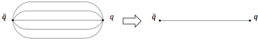
Figure 1: A simplified colour-field topology in a q\bar{q} system and its further simplified string representation.
