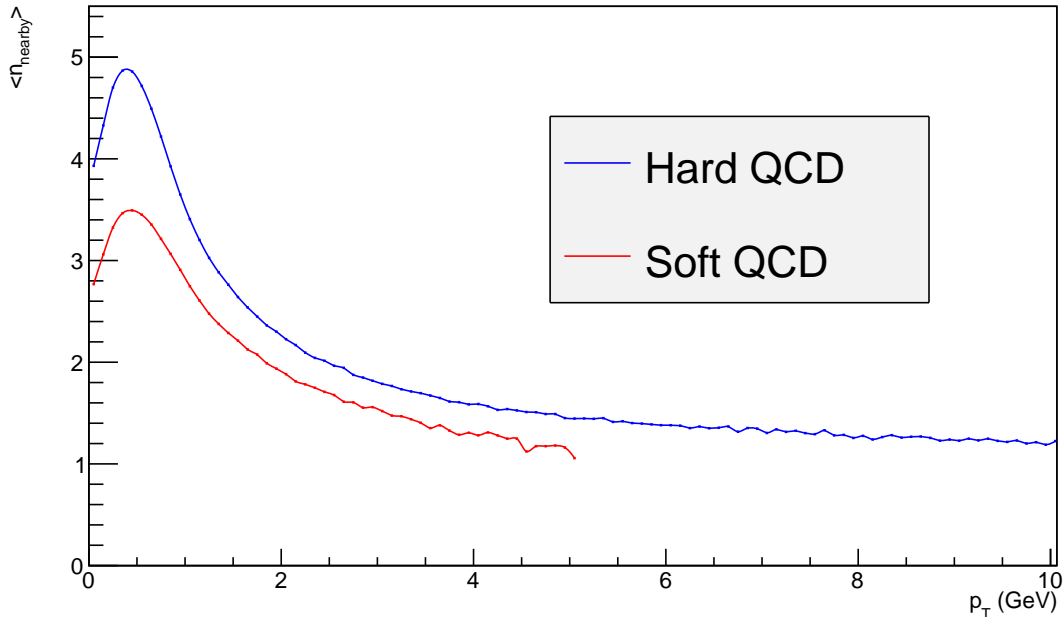
Figure 28: Average number of overlapping hadrons as a function of the p_{\perp} of the hadron studied. The red and blue distributions illustrate the soft and hard QCD processes, where the former stops at 5 GeV owing to limited statistics at large p_{\perp} .
