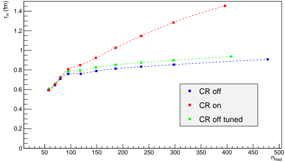
Figure 25: Median radii as a function of multiplicity for 13 TeV pp collisions. The red curve corresponds to the approach with colour reconnection, while the blue and green curves represent the model without colour reconnection and a tuned model without colour reconnection, respectively.
