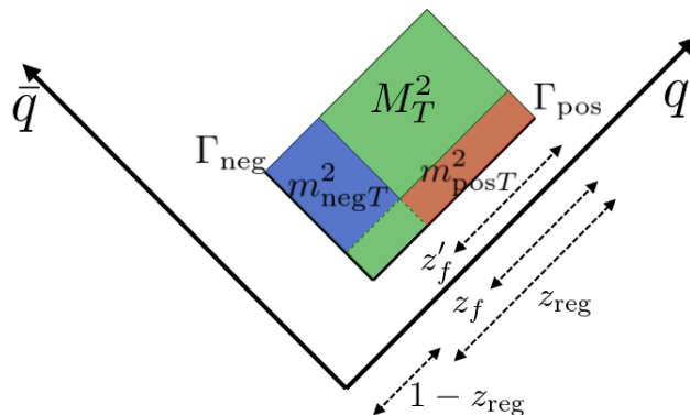
Figure 31: Final breakup and final two hadrons of a q\bar{q} system. The blue and red areas represent the two final hadrons while the green area corresponds to the final region.
