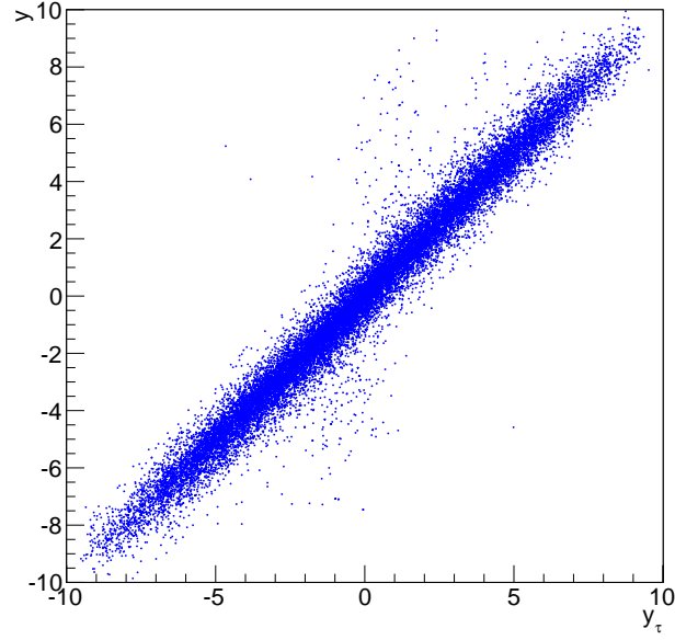
Figure 14: Correlation between rapidity, y , and the equivalent space-time rapidity, y_\tau , for all hadrons in 100 inelastic nondiffractive pp events at \sqrt{s} = 13 TeV.
