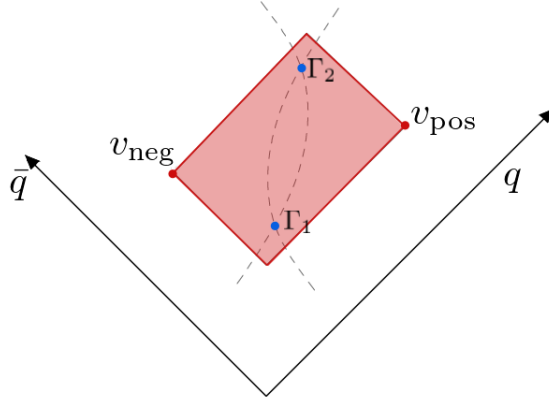
Figure 29: The two possibilities for the final breakup, in blue, and the final region, in red, in a q\bar{q} system. The two old breakups, v_{\text{neg}} and v_{\text{pos}} , are also represented in red.
