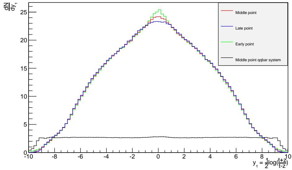
Figure 15: Longitudinal spectra for pp events and q\bar{q} systems, both at \sqrt{s} = 13 TeV.
