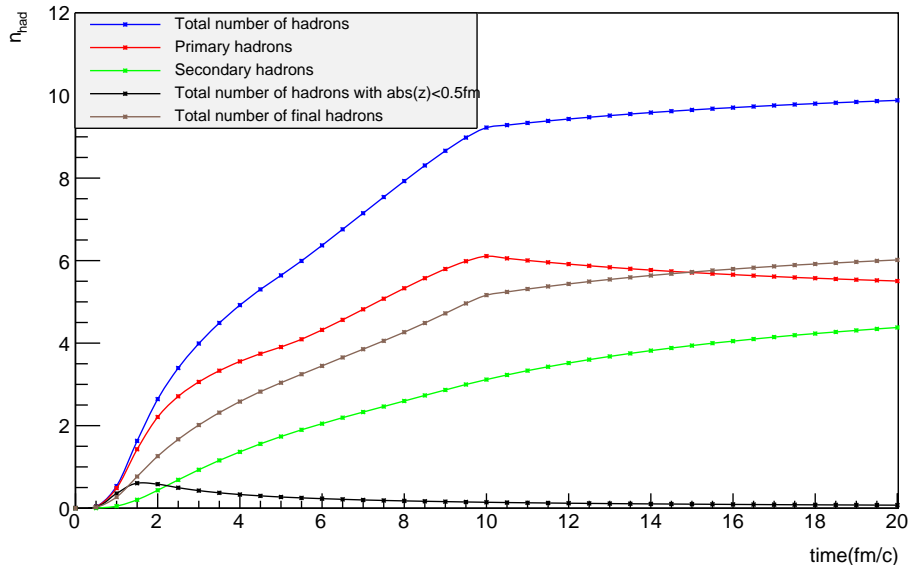
Figure 17: Hadron number per event as a function of time for a simple q\bar{q} system formed by massless quarks in the CM frame with \sqrt{s} = 20 GeV.
