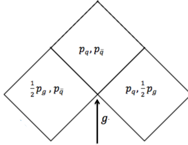
Figure 10: Parameter plane for a qg\bar{q} system.
