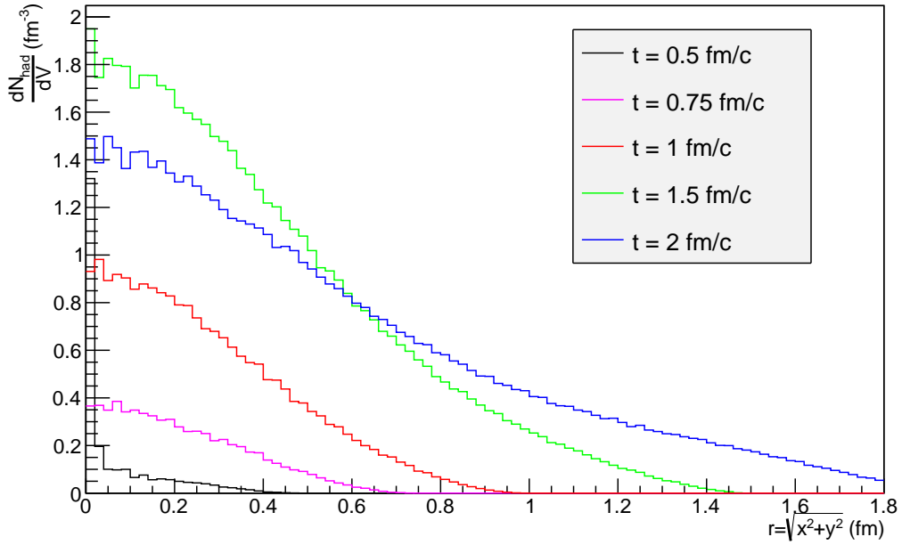
(b) 13 TeV pp collisions
