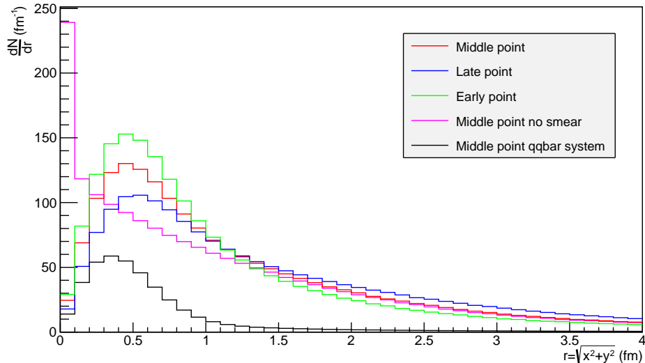
Figure 16: Transverse spectra for pp events and q\bar{q} systems, both at \sqrt{s} = 13 TeV.
