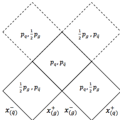
Figure 7: The parameter plane picture for the qg\bar{q} system. The dash lines indicate the turnover regions, normally neglected.
