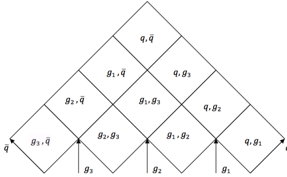
Figure 11: Parameter plane for a five parton system.
