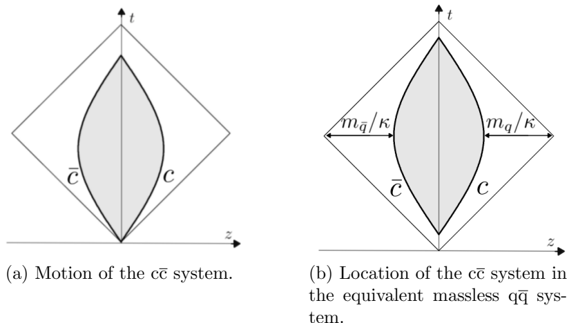
Figure 5: The c\bar{c} system and the equivalent system formed by massless q and \bar{q} .
