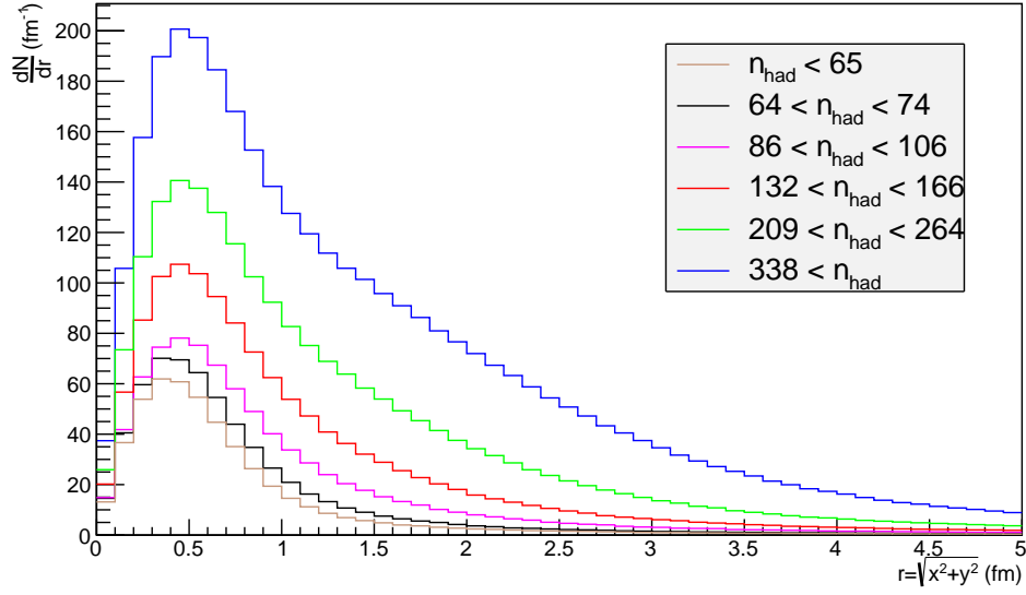
Figure 24: Transverse spectra for 13 TeV pp collisions and different multiplicity ranges.
