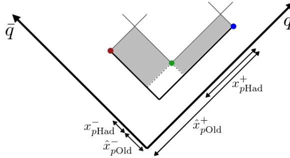
Figure 30: Final breakup point and final two hadrons, corresponding to the grey regions, in a q\bar{q} system. The red and blue points are the previous breakups and the endpoints of the final region, while the green dots represents the final breakup.
