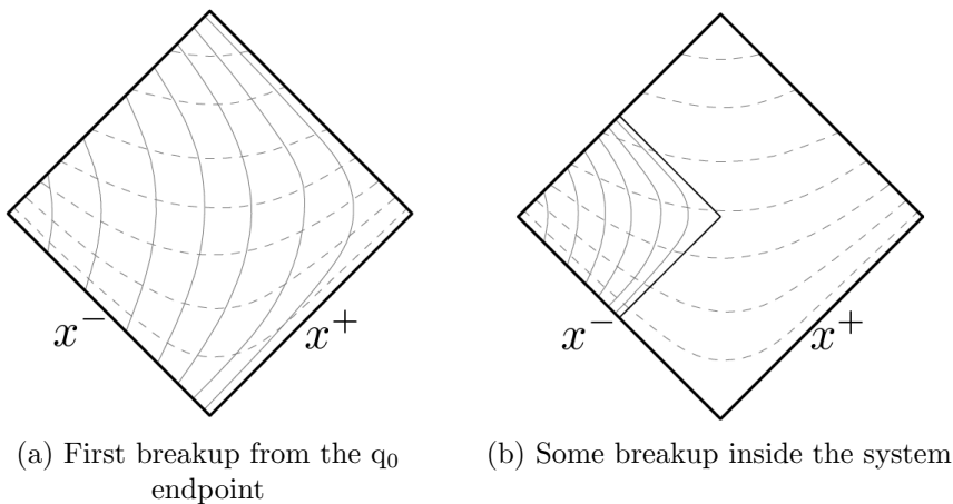
Figure 4: Hyperbolae of constant \Gamma and m_h^2 represented by dashed and full lines, respectively.
