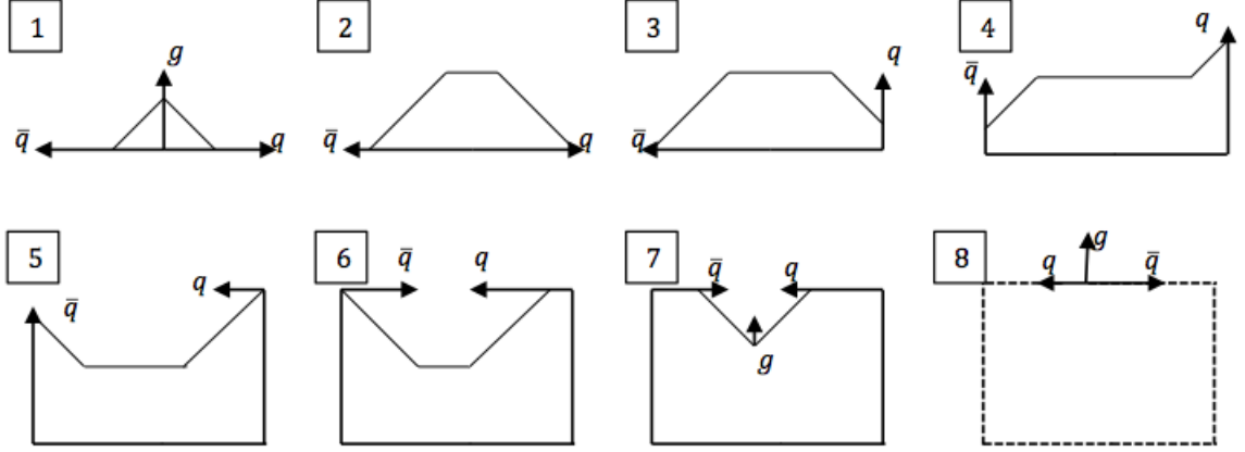
Figure 6: Time evolution of the qq\bar{q} system formed by massless partons in a frame where the gluon moves in the +x direction, while the q and \bar{q} move in opposite directions along the z axis.
