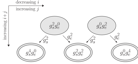
(a) We consider the coupling-power combinations g_s^i g_e^j at the amplitude level. From left to right we have increasing i / decreasing j in steps of 2. From top to bottom the total order i+j increases in steps of 2. The upper row depicts all possible coupling-power combinations for the lowest-order contributions, with i+j=n-2 , while the lower row depicts all possible coupling-power combinations for the higher-order corrections of one loop order higher, with i+j=n .
