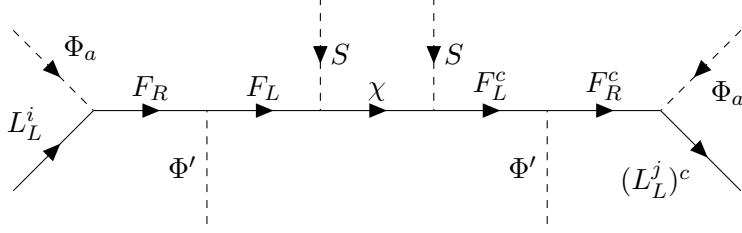
Figure 1: A diagram generating the ij -element of the Weinberg operator, \chi is a Majorana fermion with mass \sim \Lambda_{FN} . Here the four-component spinor Feynman rules from ref. [24] are used.
