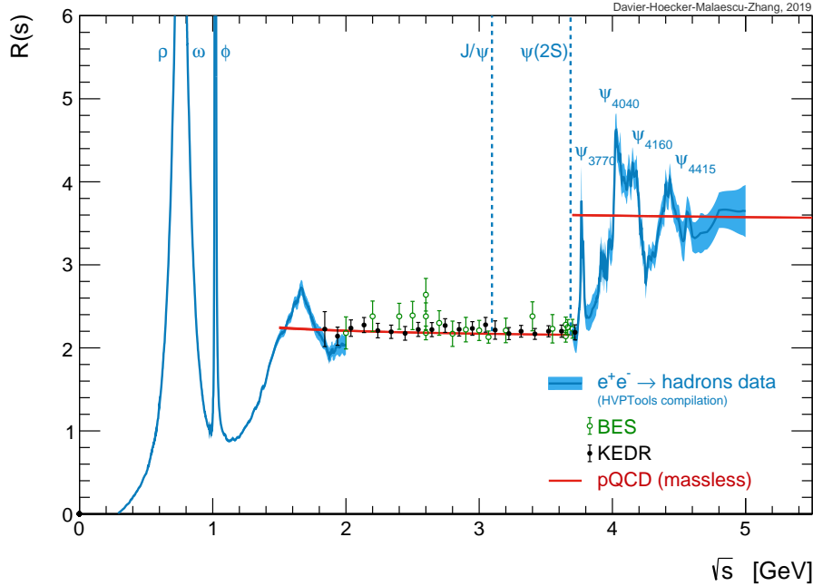
Figure 12: The total hadronic e^+e^- annihilation cross section ratio R as a function of \sqrt{s} [2]. Inclusive measurements from BES [37, 41, 59] (and references therein) and KEDR [75, 86, 164] are shown as data points, while the sum of exclusive channels from this analysis is given by the narrow blue bands. Also shown is the prediction from massless pQCD (solid red line). Reprinted from Ref. [6].
